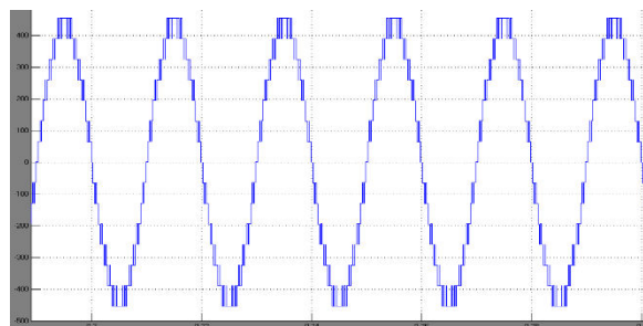
Fig.9 Output wave for 18 switch MLI inverter output voltage with 15 level of waveform
