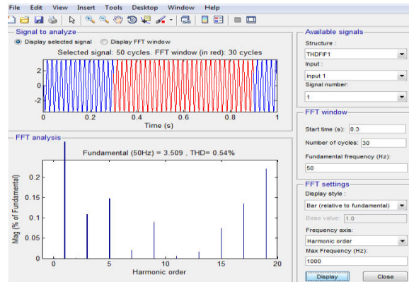
Fig.10 Assuming that the stages are expanded past 5, the THD will be better for second plan with RV.
