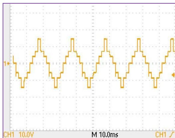
Fig.12 Output wave form 5 Level MLI
