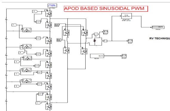
The figure. 8 proposed model with APOD pulse width modulation technique with RV system
